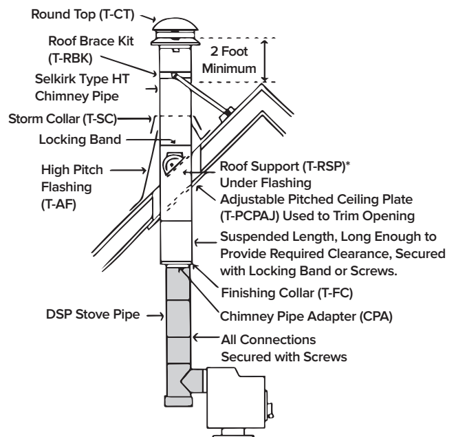
⑧ A-Frame with Chimney on a Steep Pitch Roof
