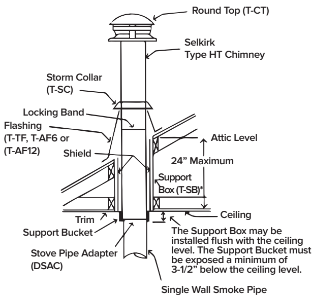
⑦ Pitched Roof with Attic
