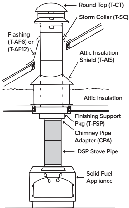
④ Solid Fuel Appliance with a Short Vertical Chimney
